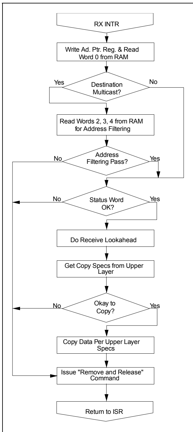
Figure 5.4 - RX INTR
